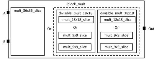
Fig. 6.6: Model of a fracturable multiplier block
